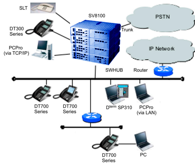
Figure 1-7 Simplified SV8100 System (9.5' Base and Expansion) Connectivity
